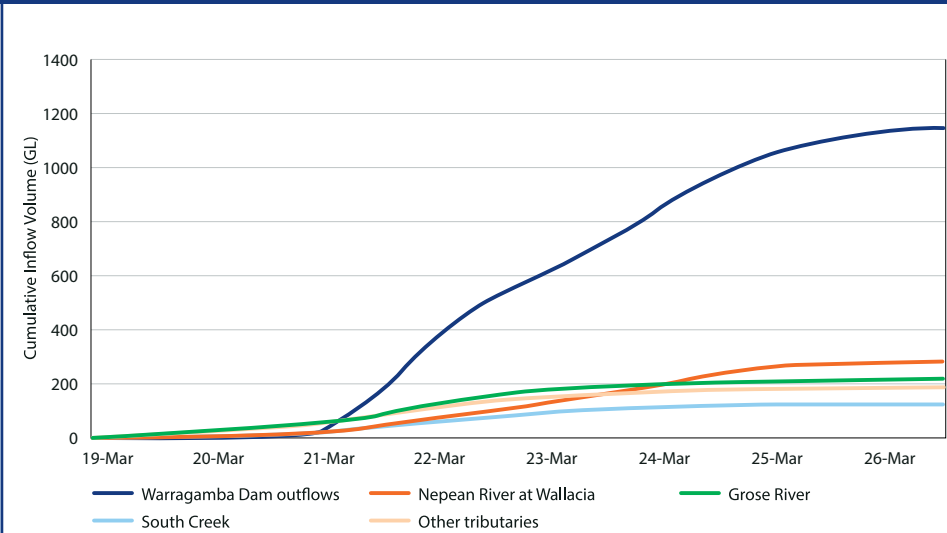
Figure 10: Cumulative inflows to Windsor, March 2021 flood
