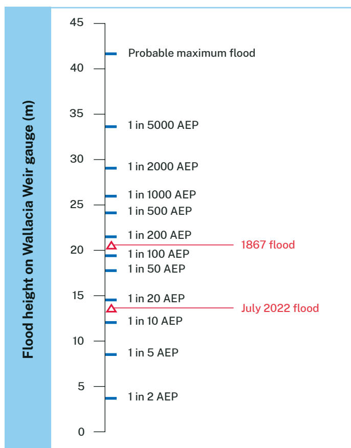
Potential flood heights compared to 2 historical floods, Wallacia Weir
