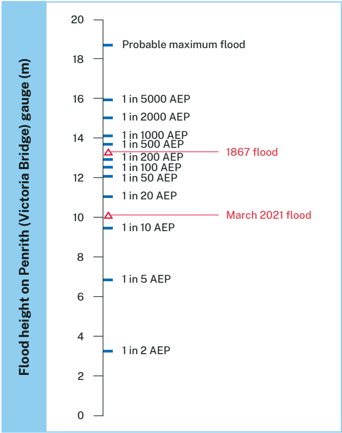
Potential flood heights compared to 2 historical floods, Penrith
