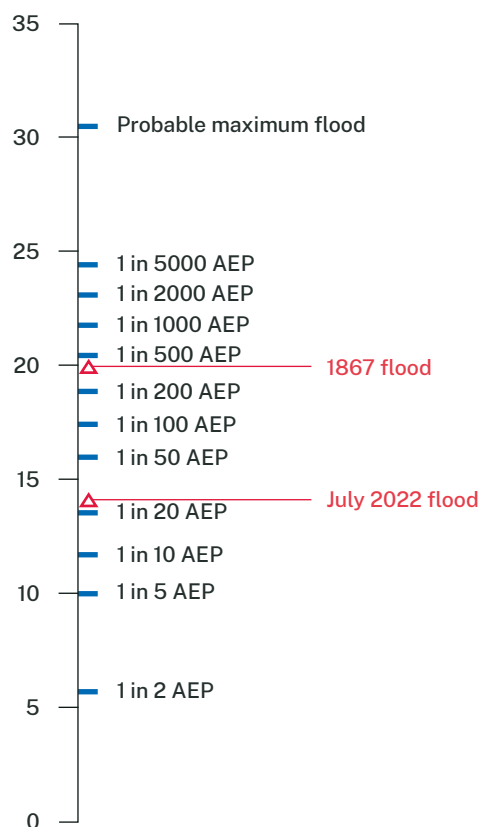
Flood height on Windsor PWD gauge (m AHD)
