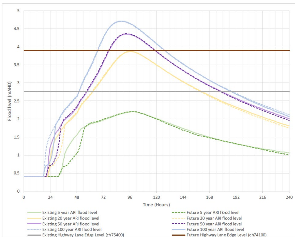
Figure 11: Road height and overtopping level and duration of the Pacific Highway– south of Shark Creek (27).
